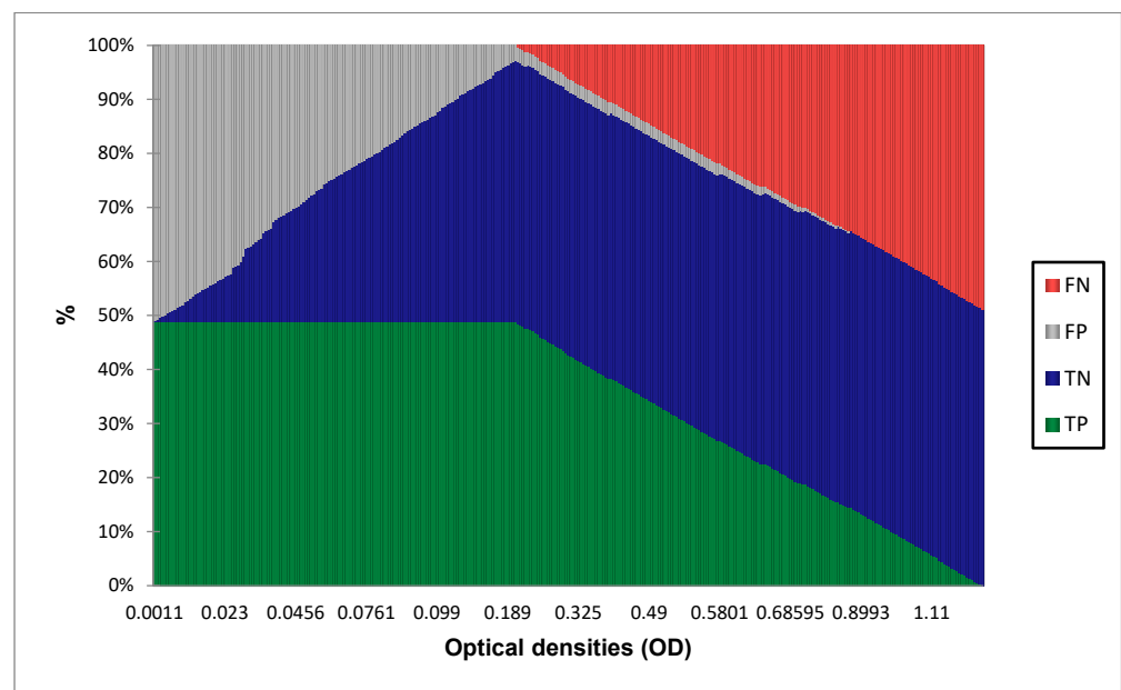
Figure 3. True positive (TP), true negative (TN), false positive (FP), and false negative (FN) proportions.
